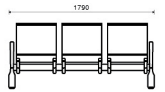
Model. FLITE-03
