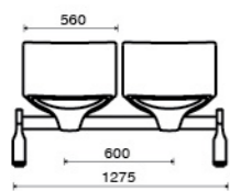
Model. TURINI-02
