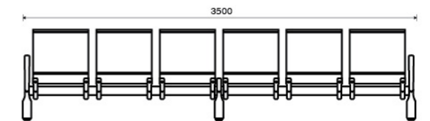
Model. FLITE-06
