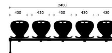
Model. MOTO 05
